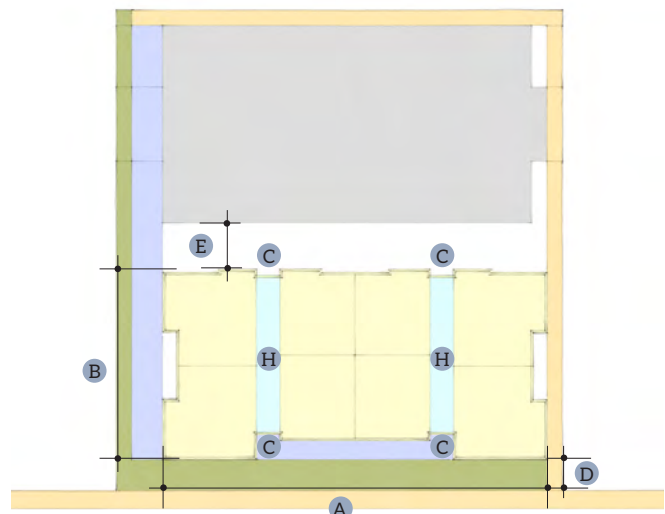
Figure 2.90 Example of Double-Aspect Walk-Up Multiple-Family Building
